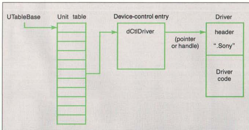
Figure 1: Finding a driver. UTableBase points to the unit table that contains handles to device-control entries. The DCE references the actual driver.
